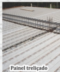
Painel treliçado
